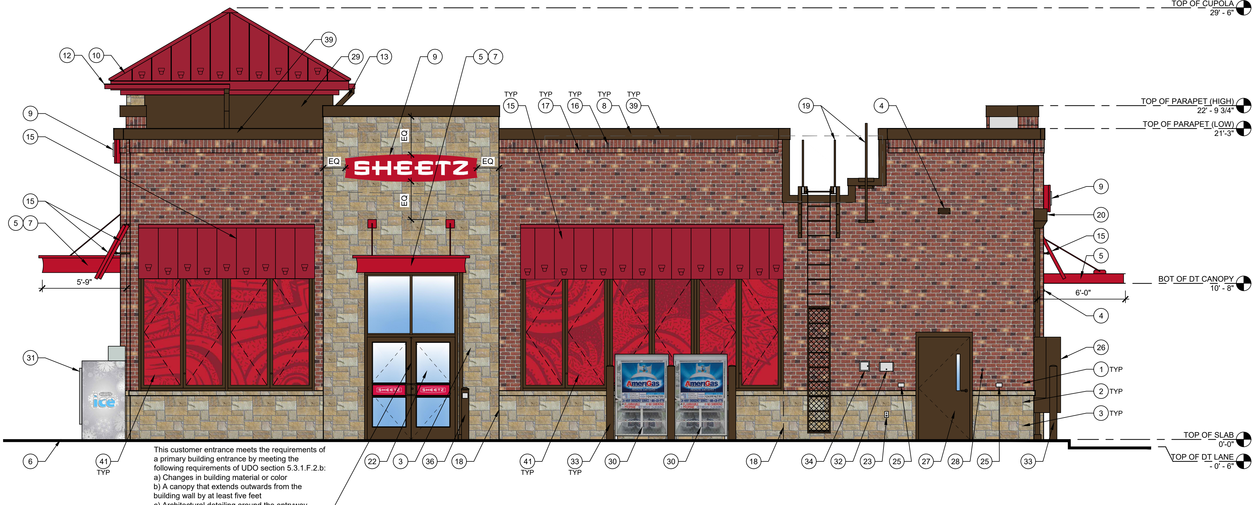
4 RIGHT ELEVATION 1/4" = 1'-0"
